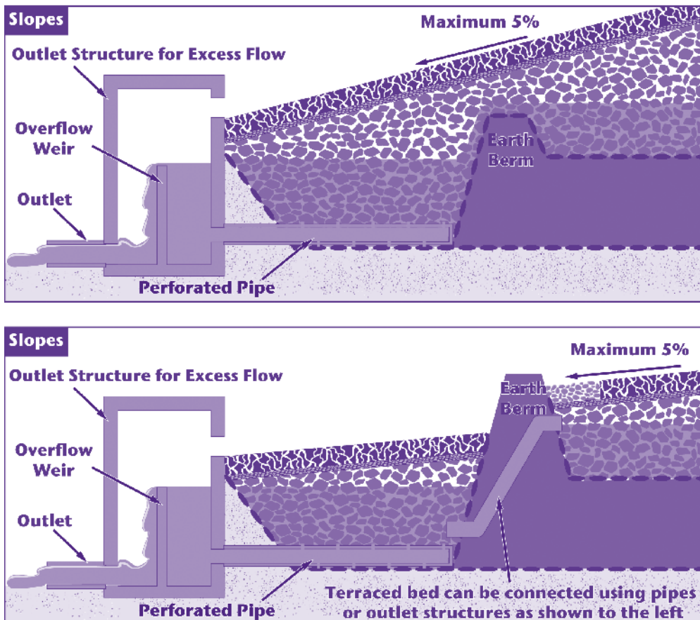
Figure 4: Terraced porous parking
