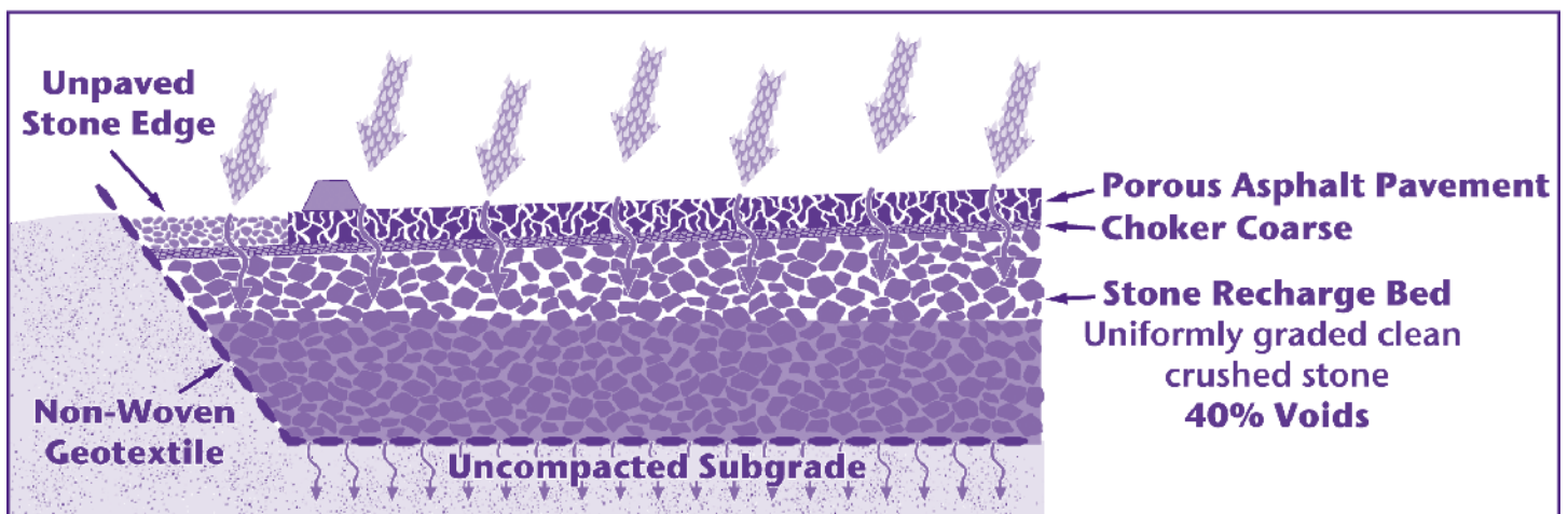
Figure 1: Typical Porous Pavement Cross Section
